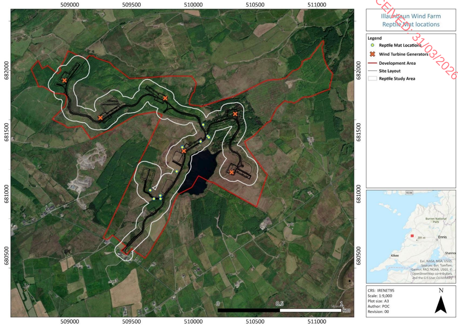
Figure 2.3: Illeunbaun Wind Farm Reptile mat locations and Study Area.
